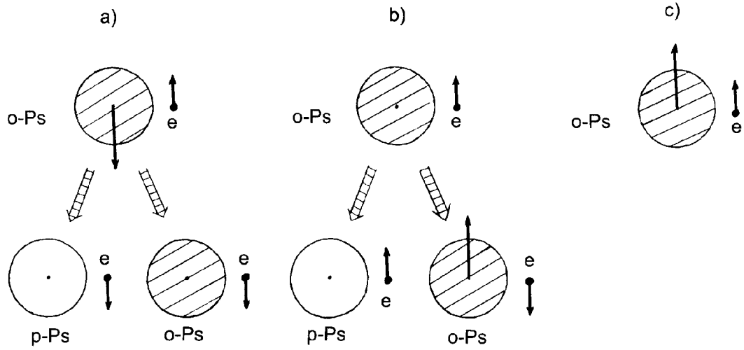
Figure 1. Spin-conversion of the o-Ps: a) the o-Ps (hatched) with the spin projection S_z = -1 can convert either into the p-Ps (white) or into the o-Ps with S_z = 0 ; b) the o-Ps with S_z = 0 can convert either into the p-Ps with S_z = -1 or into the o-Ps with S_z = 1 ; c) the o-Ps with S_z = 1 cannot convert.
