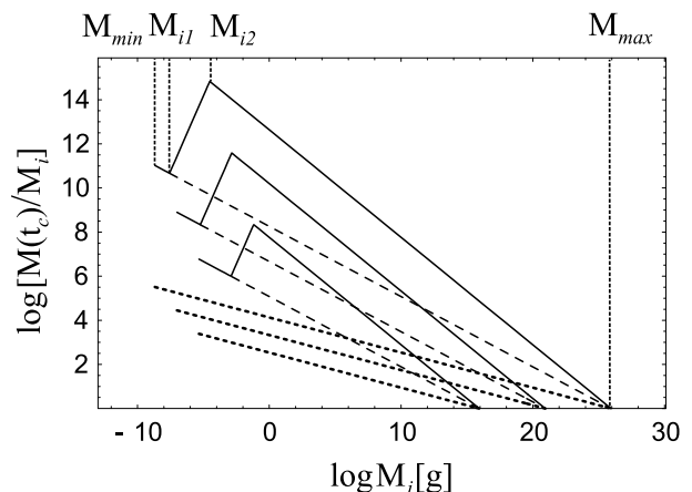
FIG. 1: Accretion mass growth coefficient vs the initial PBH mass for choices l/l_4 = 10^{21}, 10^{26} and 10^{31} (from bottom to top). Solid lines correspond to the PBH mass growth coefficient (30), while long dashed and short dashed ones are obtained from Eq. (6) with fixed accretion efficiencies F = 1 and F = 0.5 , respectively.
