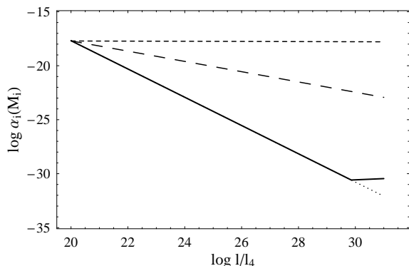
FIG. 2: Constraints on initial PBH mass fraction imposed by the total matter density. Dotted, long dashed and short dashed lines are obtained using PBH mass growth coefficient (6) with F = 1.54, 1 and 0.5 , respectively.
