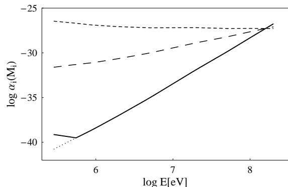
FIG. 3: Constraints on initial PBH mass fraction imposed by the high-energy diffuse photon background. Dotted, long dashed and short dashed lines are obtained using Eq. (6) with F = 1.54, 1 and 0.5 , respectively.
