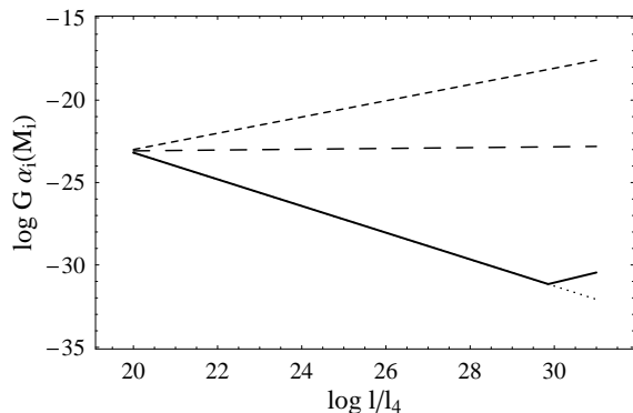
FIG. 4: Constraints on initial PBH mass fraction imposed by the antiproton excess. Dotted, long dashed and short dashed lines are obtained using Eq. (6) with F = 1.54, 1 and 0.5 , respectively.
