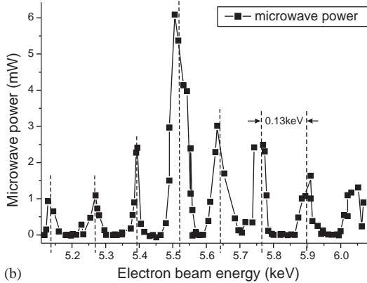
Fig. 1. (a) General view of microwave signal. (b) Dependence of microwave power on electron beam energy.
