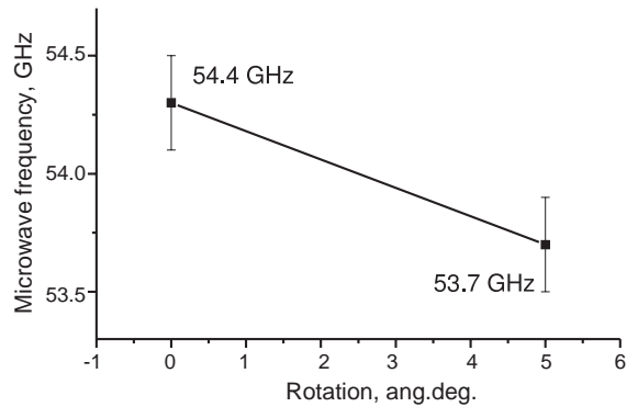
Fig. 3. Measured frequencies at rotation of resonant diffraction grating.
