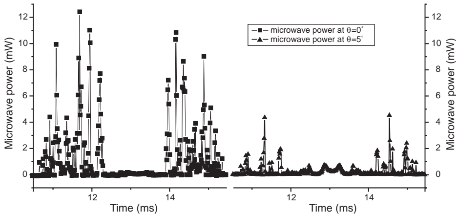
Fig. 2. Change of lasing efficiency with grating rotation, \theta is the angle of grating rotation, \theta = 0 when grating grooves are perpendicular to e-beam velocity.
